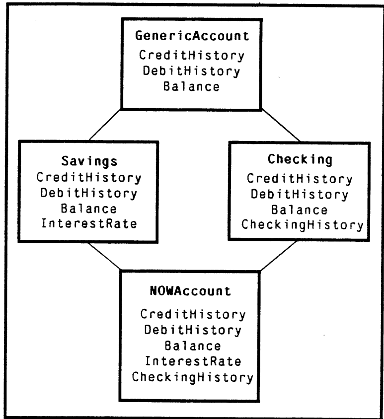
Figure 6.1. Inheritance lattice for Bank Account example
